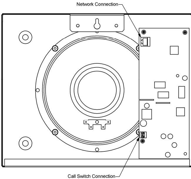
FIG 1. VIP-430 CONNECTIONS
