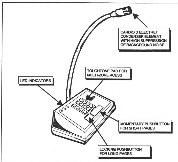
Figure 1. Multi-Zone Microphone Features
