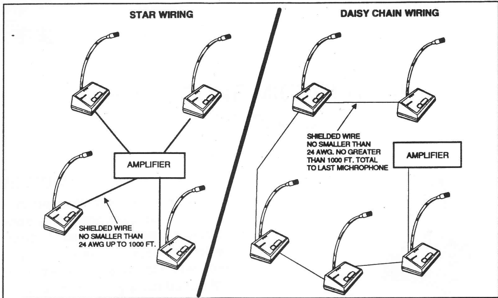
Figure 4. Star or Daisy Chain Wiring Configurations
