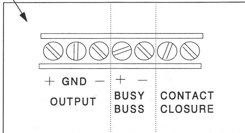
Figure 3. Wiring Connections on Microphone Terminal Block
