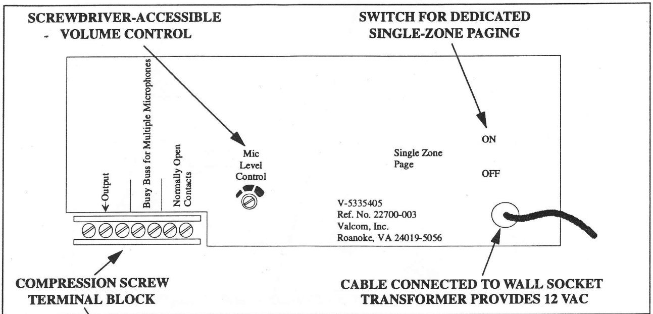
Figure 2. Back Panel Controls and Connectors
