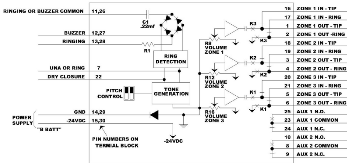
FIGURE 3 – SIMPLIFIED SCHEMATIC
