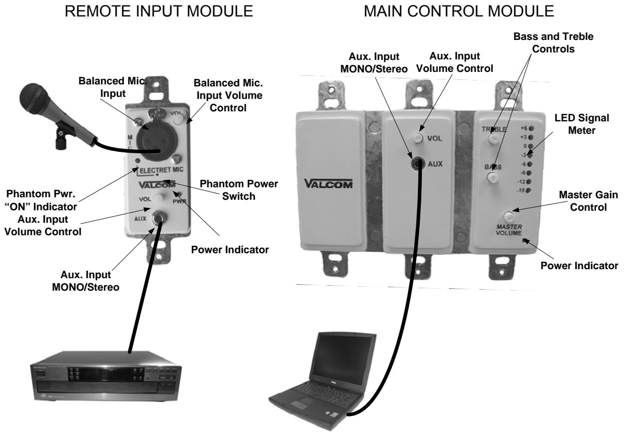
Figure 3: Typical Connections
