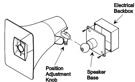
Figure 2 - Mounting to an Electrical Backbox
