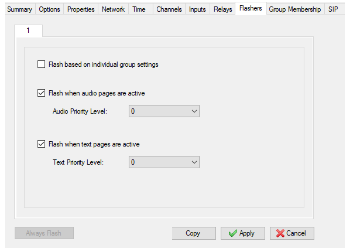
Figure 135: Flashers Tab Dialog Box
