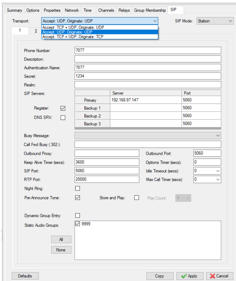
Figure 143: SIP Tab Using SIP Mode Station Dialog Box
