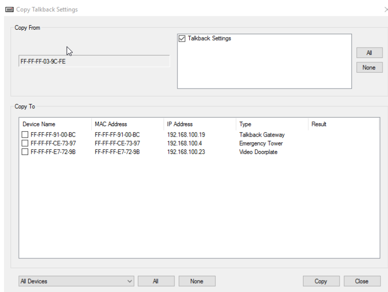
Figure 114: Copy Talkback Settings Dialog Box
