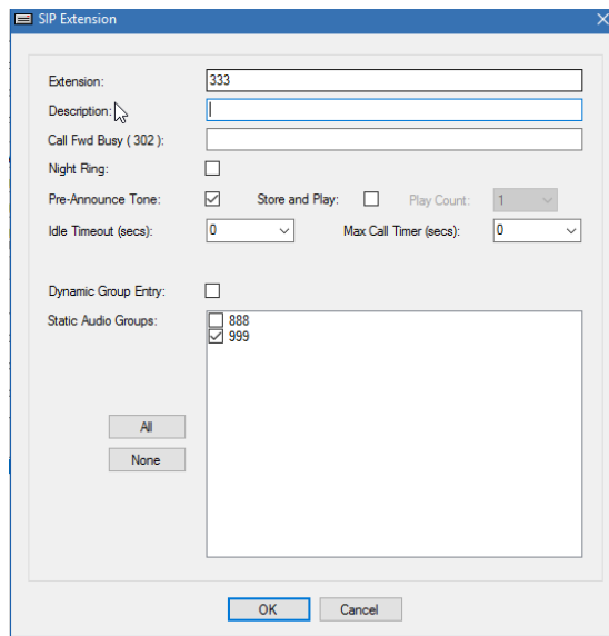
Figure 145: SIP Tab Using SIP Trunk Mode Adding Extensions Dialog Box
