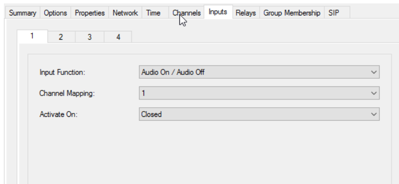
Figure 120: Inputs Tab Using Audio On /Audio Off Function Dialog Box
