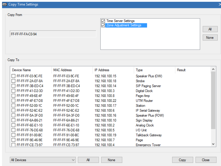
Figure 111: Copy Time Settings Dialog Box
