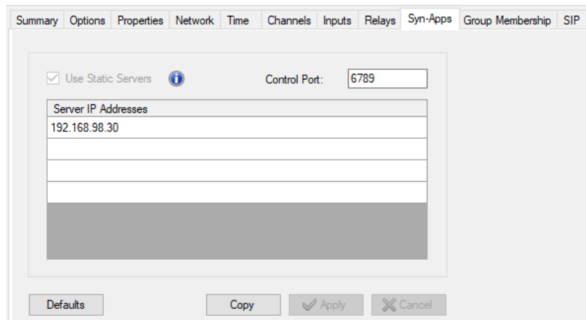
Figure 138: Syn-Apps Tab Dialog Box
