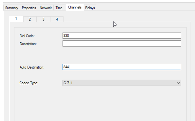
Figure 119: Channels Tab for VIP-854 Device Dialog Box
