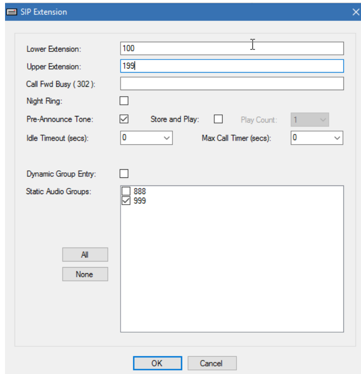
Figure 146: SIP Tab Using Trunk Mode Adding Extensions Dialog Box
