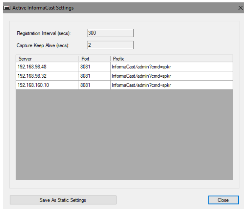
Figure 106: Active InformaCast Settings Dialog Box
