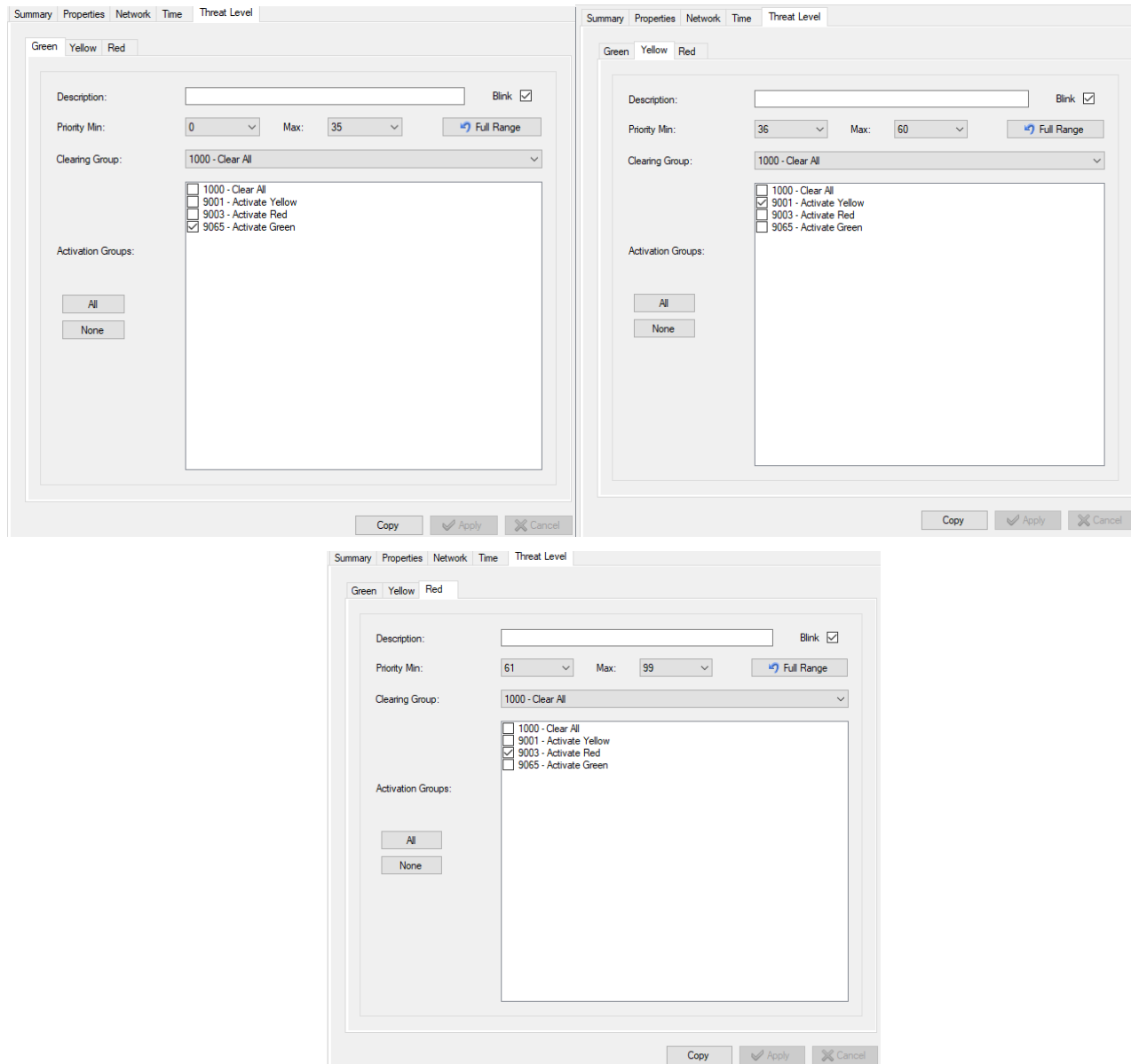
Figure 112: Threat Level Tab Dialog Boxes
