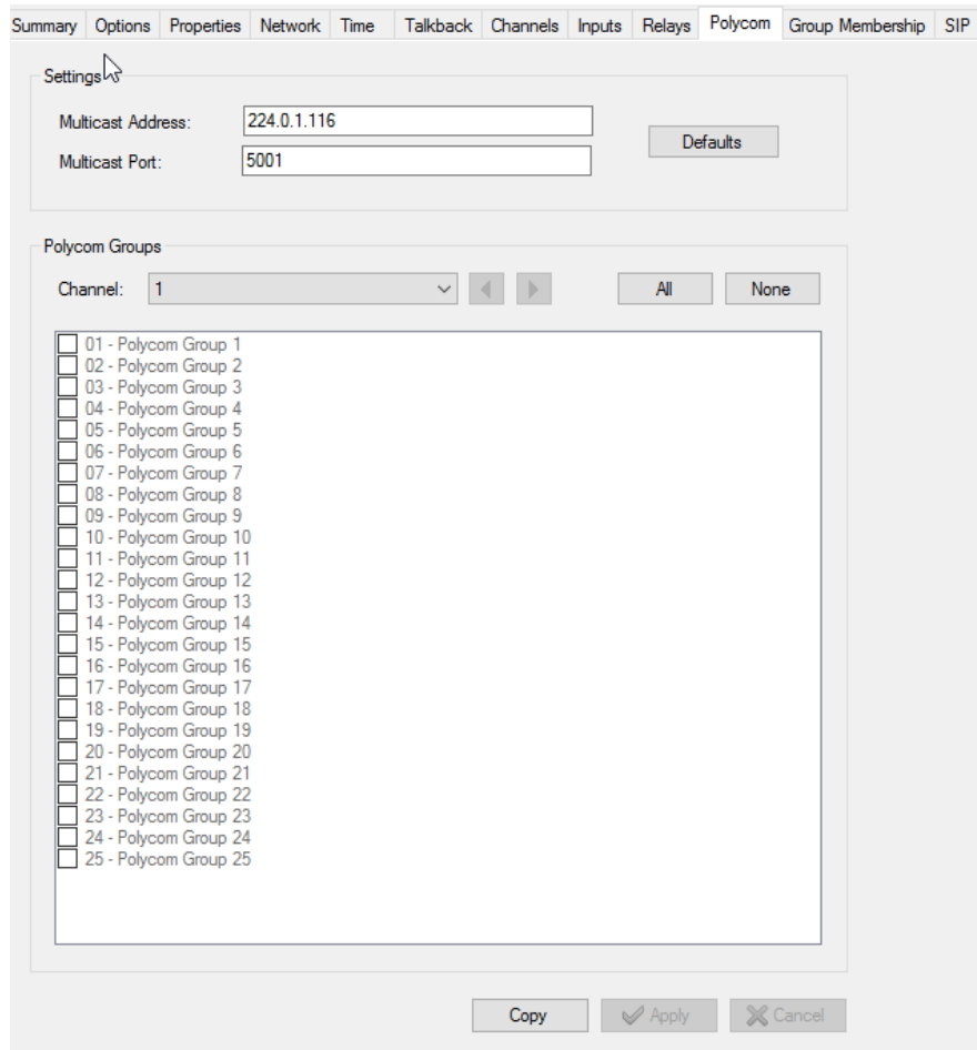
Figure 139: Polycom Tab Dialog Box
