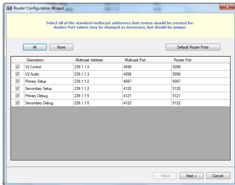
Figure 151: Router Configuration Wizard Dialog Box
