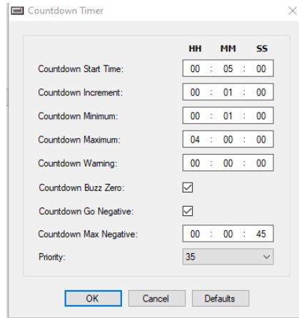
Figure 133: Countdown Timer Dialog Box
