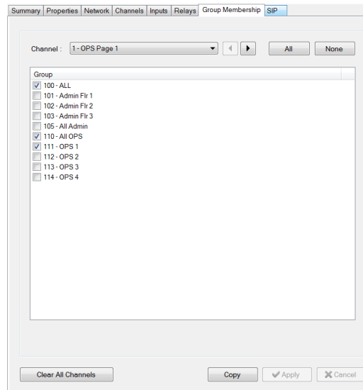
Figure 141: Group Membership Tab Dialog Box
