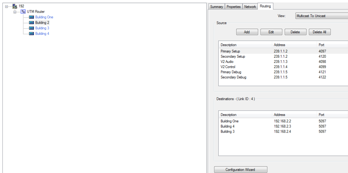
Figure 150: Routing Tab Dialog Box
