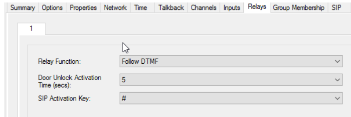
Figure 127: Relay Tab for Talkback Speakers Dialog Box
