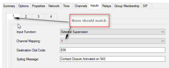
Figure 121: Inputs Tab Using External Supervision Function Dialog Box
