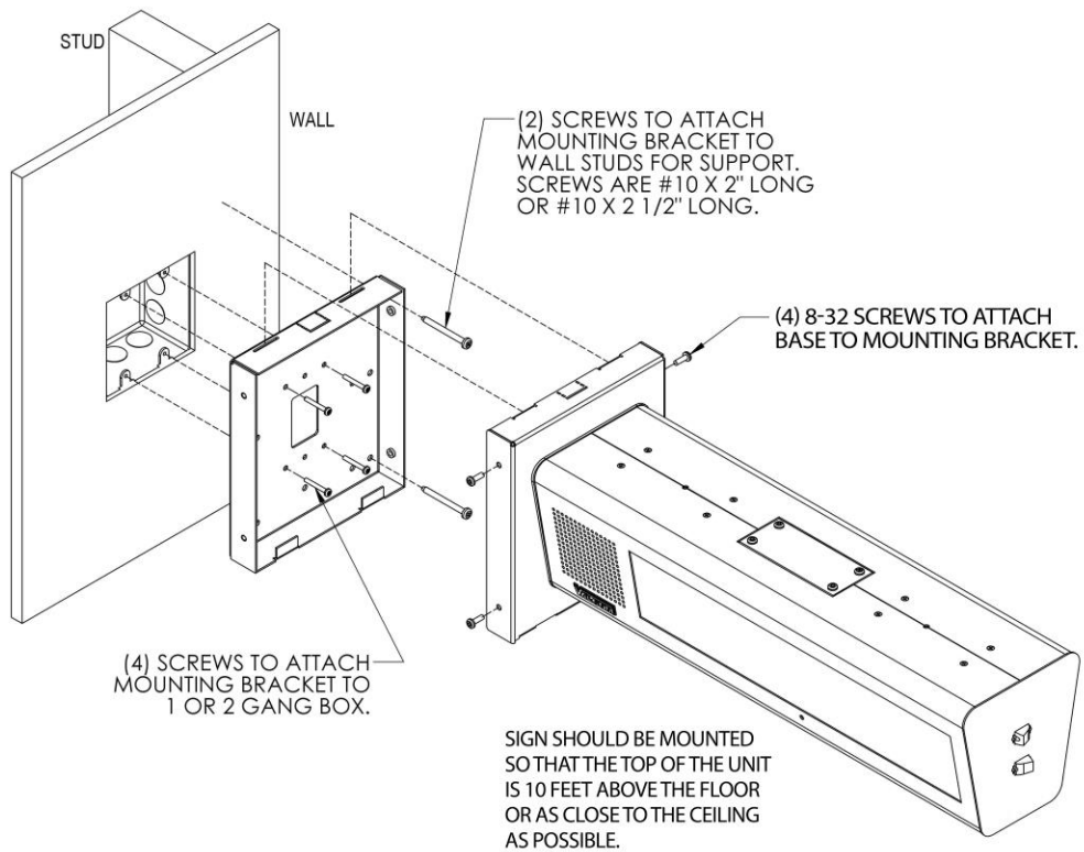
Figure 2. Wall Mount
