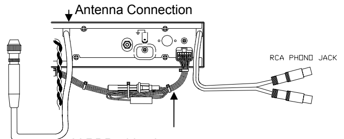
V-RDP wiring harness FIGURE 3
