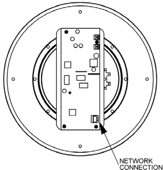
Figure 1. VIP-120 Connections
