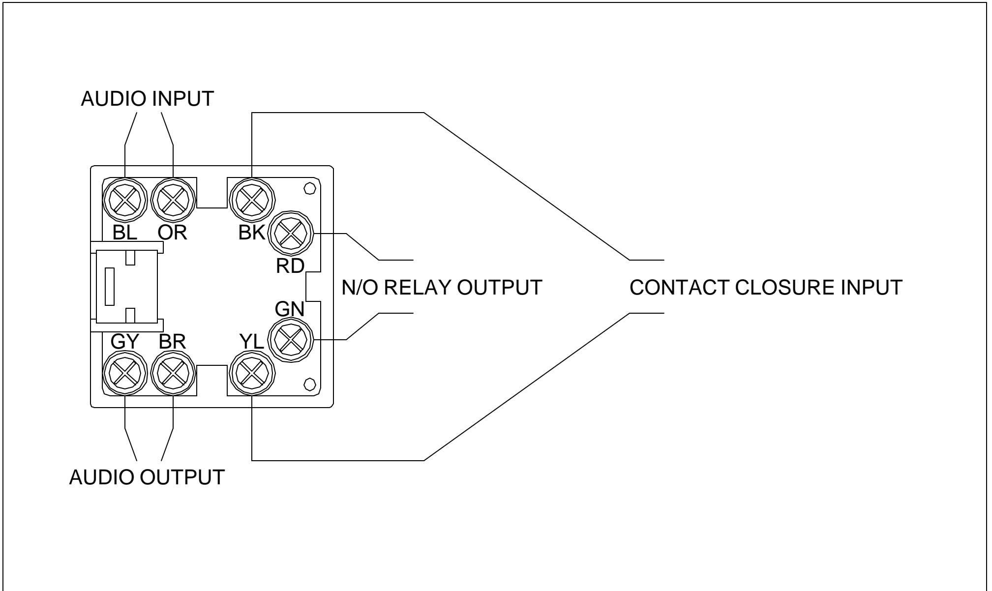
*FIGURE X = VIP-802 and VIP-804 Pinouts*
