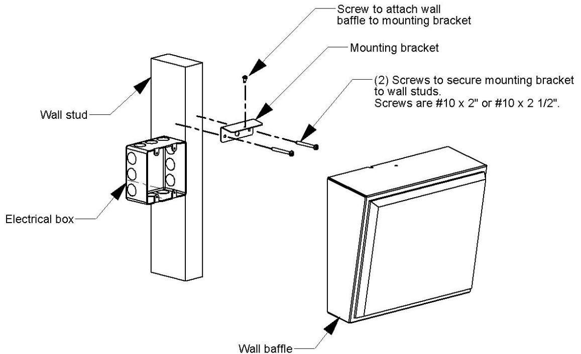
Figure 5. Speaker Mount
