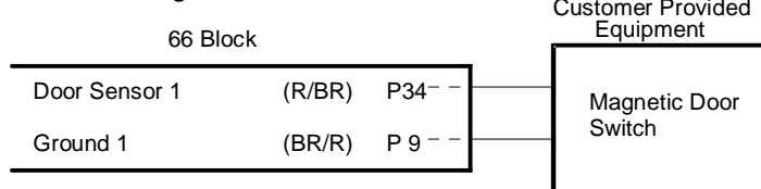
Figure 9 - Door Sensor
